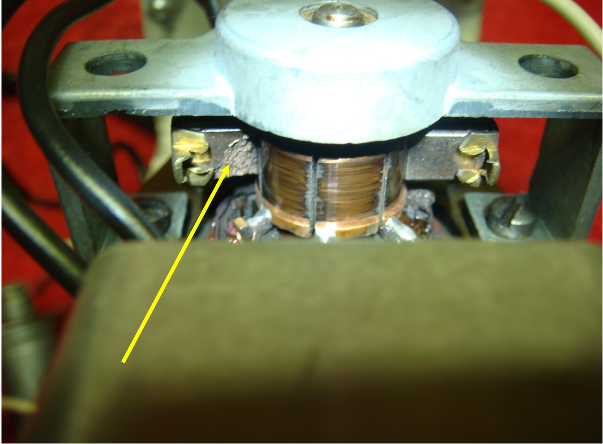
Note condition of brushes -- they may require replacement
