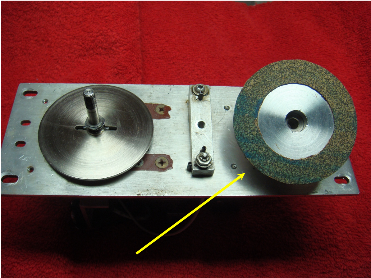
Stock cork gasket used to make clutch plate with aviation adhesive
